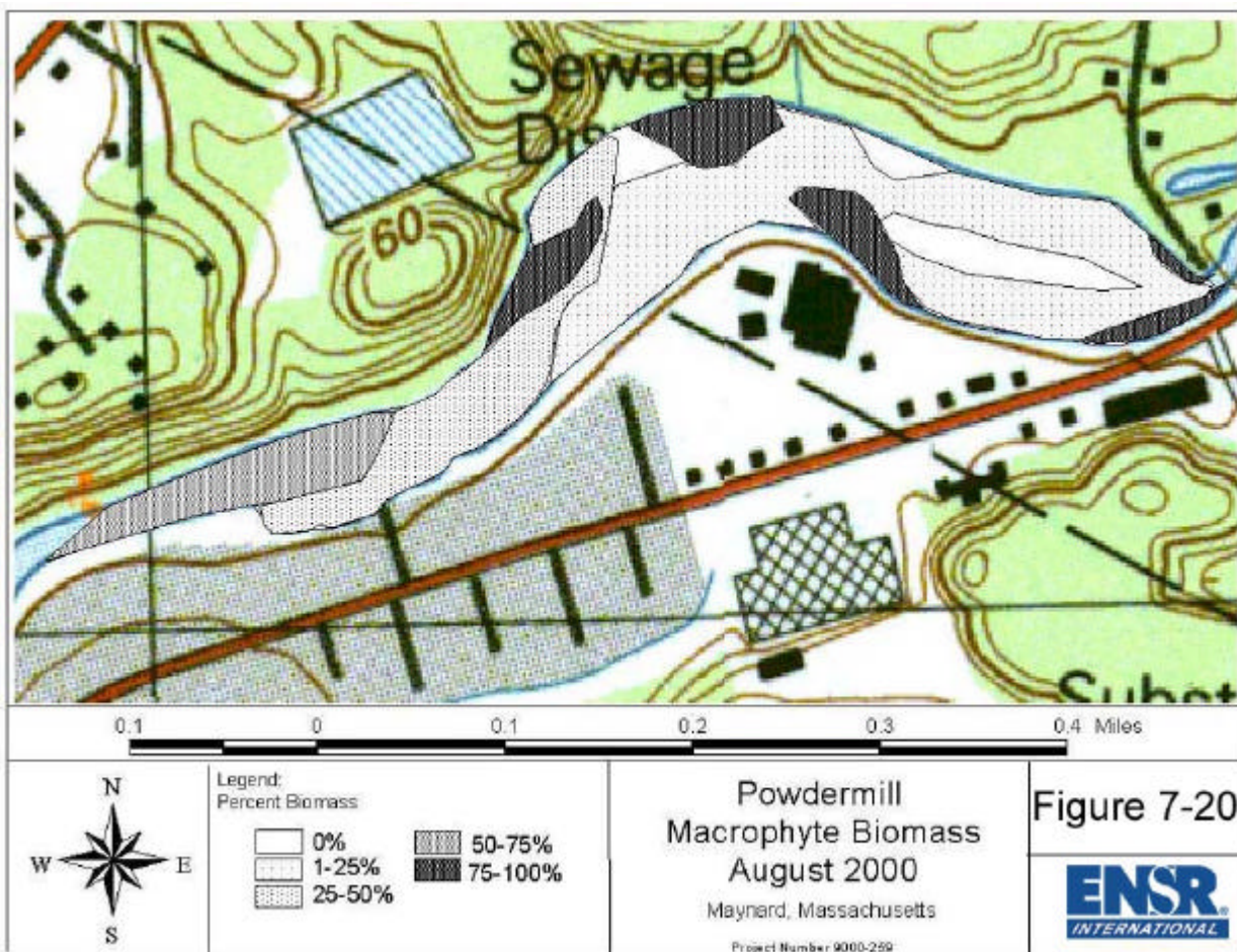
Figure 7-27 Powdermill Macrophyte Biomass, August 2000
